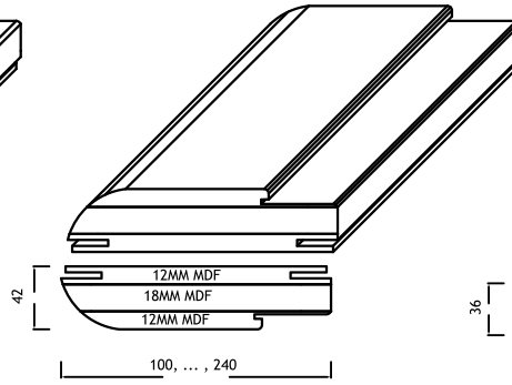
5 NOLU TAM RADIUS KASA 5. no radius frame
