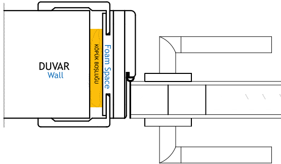
YAN PERVAZ - KASA DETAYI Side Architraves - Frame Details
