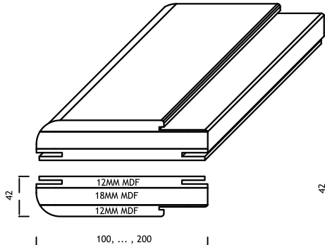
4 NOLU YARIM RADIUS KASA 4. no half radius frame
