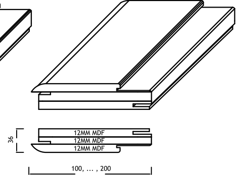
6 NOLU ÖZEL RADIUS KASA 6. no special radius frame
